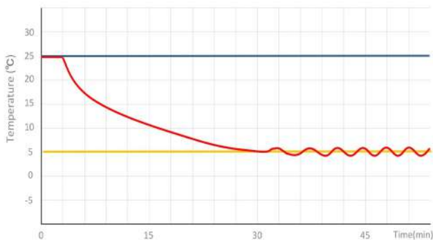
MPC-5V60G Pull Down Curve
